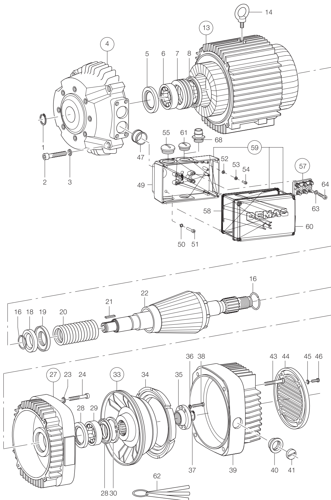
Motor KBH 140 B2/12
