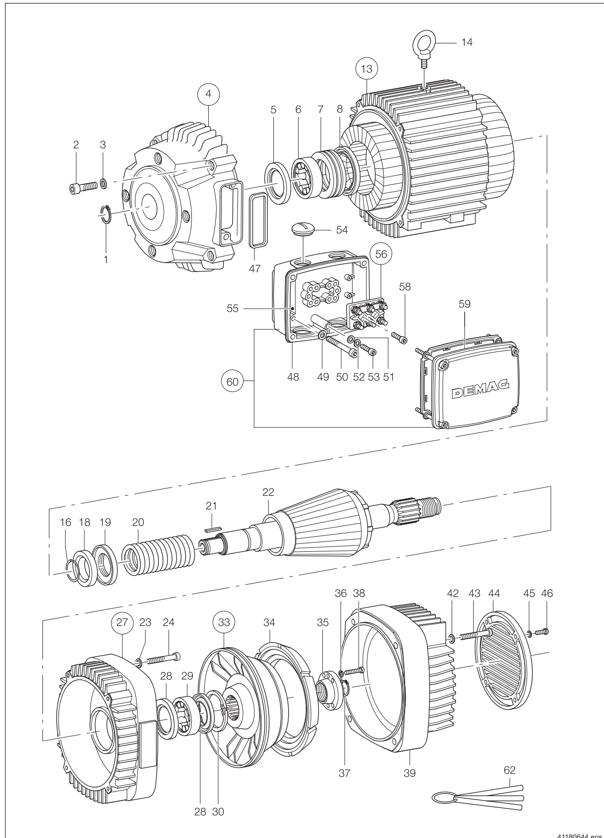
Motor KBH 125 B4
