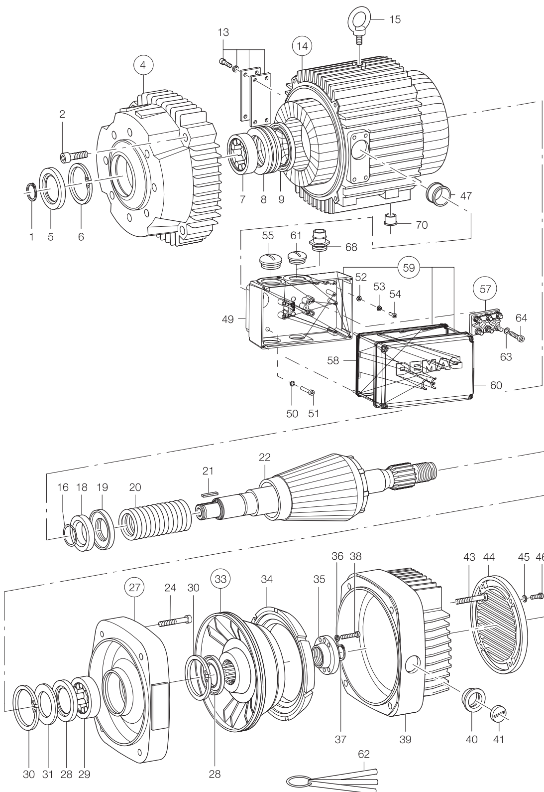
Motor KBH 200 B2/12
